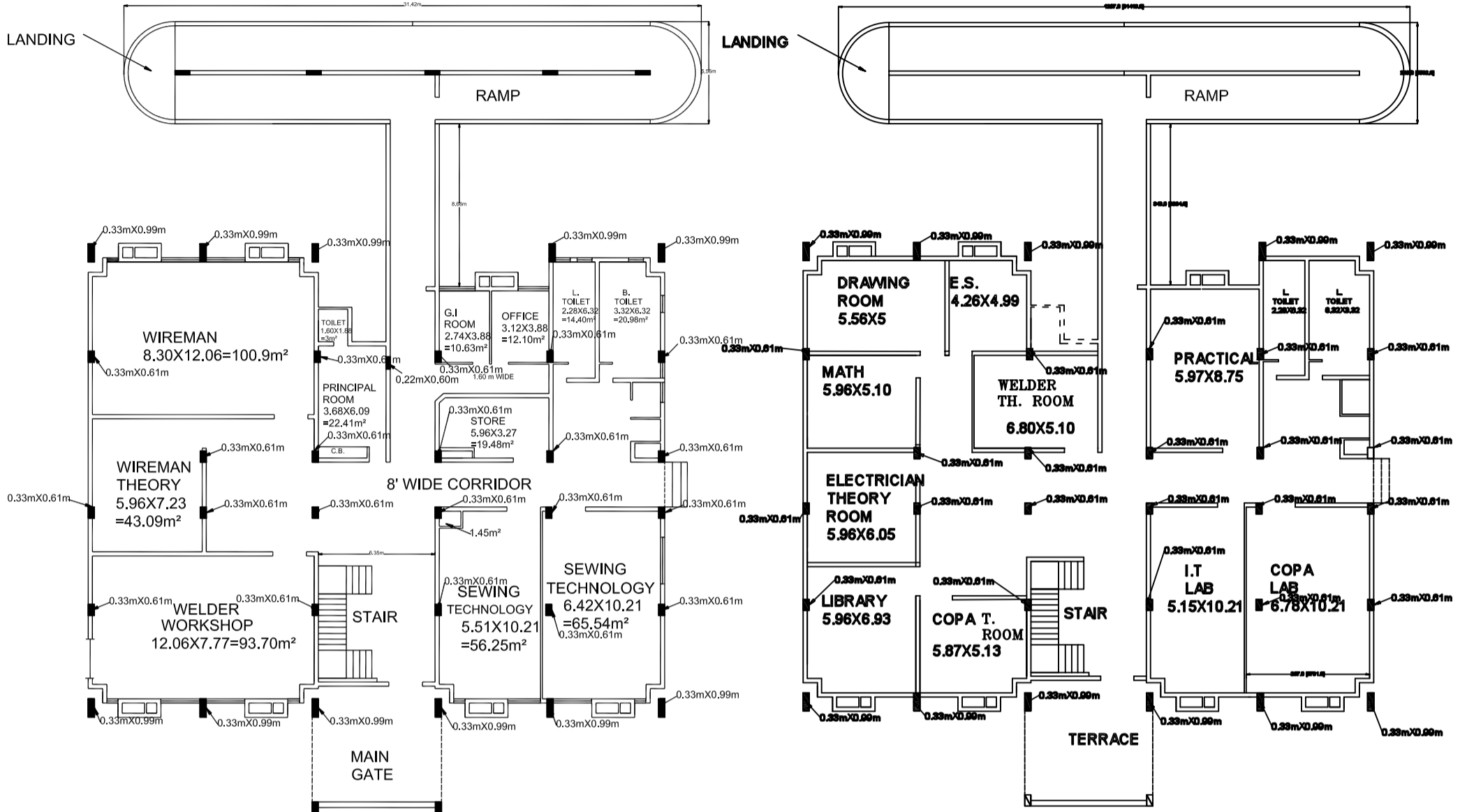
GROUND FLOOR PLAN G.I.T.I MAUJABAD
